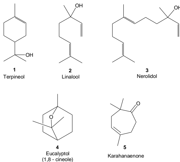
Fig. 1. Chemical structures of terpenic alcohol and its natural derivatives
