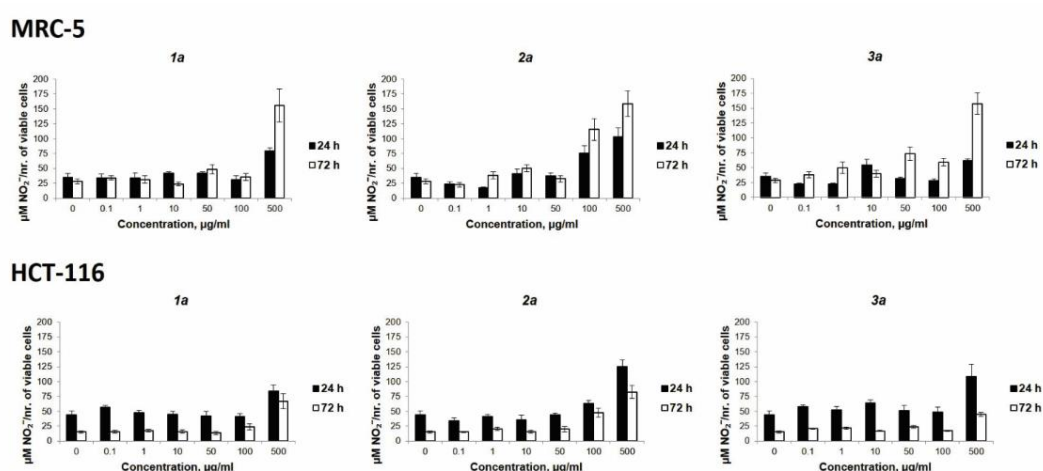
Fig. 6. Effects of 1a , 2a , and 3a on HCT-116 and MRC-5 cell lines, expressed as the NO_2^- concentration after 24 h and 72 h of exposure
