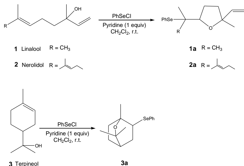
Fig. 2. Cyclofunctionalization of linalool, nerolidol, and \alpha -terpineol with PhSeCl in the presence of pyridine
