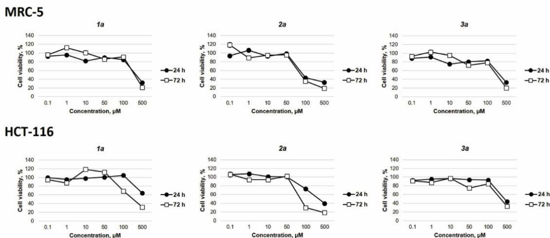
Fig. 3. Cell viability after 24 h and 72 h of exposure, expressed in percentages of viable cells
