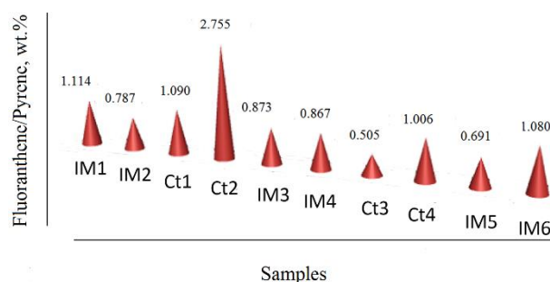
Fig. 6. Column diagram showing the distribution of the fluoranthene/pyrene ratio in different sediment (IM and Ct) samples
