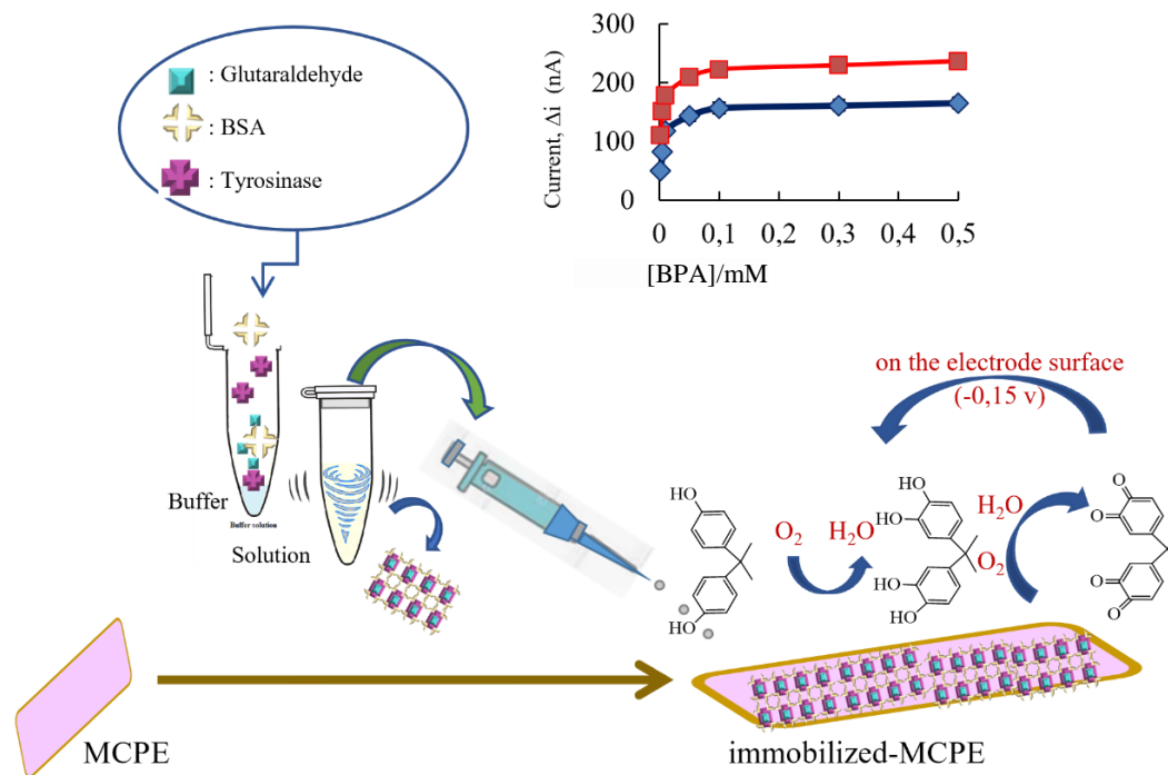
Fig. 3. Operation scheme of the BPA biosensor
