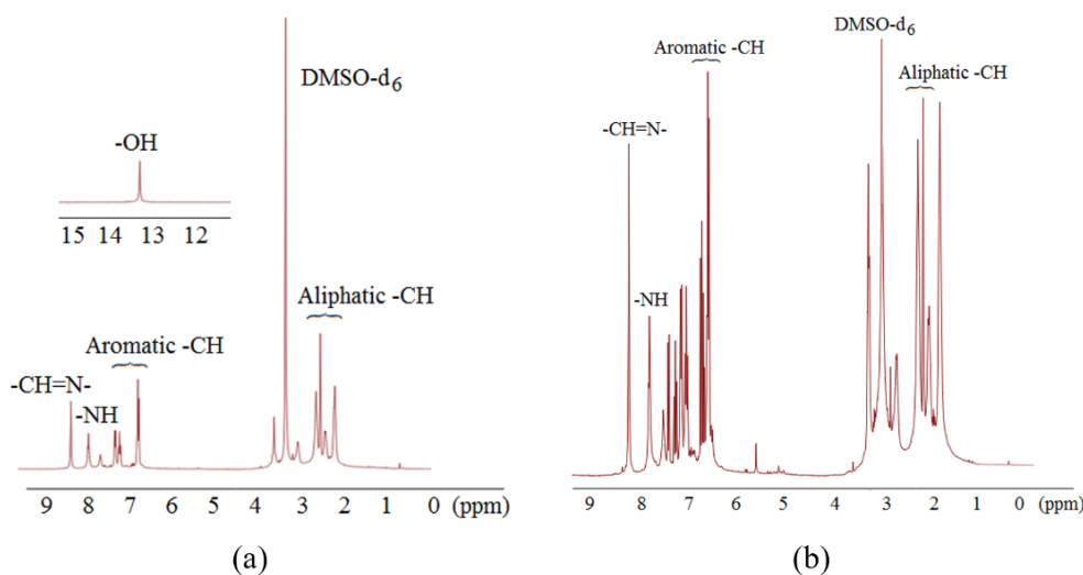
Fig. 5. 1 H-NMR spectrum of (a) PAMAM-Sal and (b) PAMAM-Sal-Pt(II)
