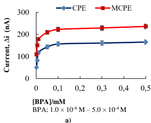
Fig. 6. (a) Amperometric response of CPE and MCPE to BPA. (b) Effect of working potential on the BPA sensitivity of MCPE (0.1 M, pH 7.0 phosphate buffer, 25 °C)
