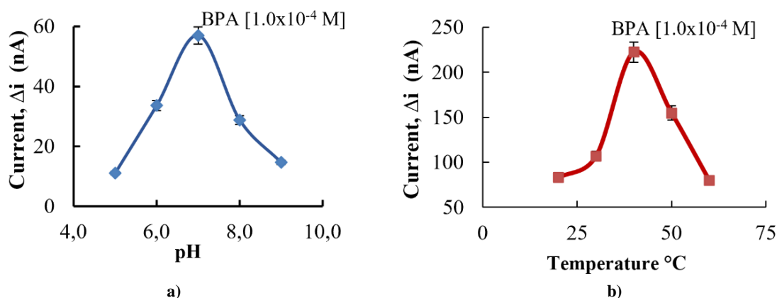
Fig. 8. (a) Effect of pH on the response of the biosensor (25 ^{\circ}\text{C} , 1.0 \cdot 10^{-4} \text{ M} BPA) (b) Effect of temperature on the response of the biosensor (pH 7.0 PBS, 1.0 \cdot 10^{-4} \text{ M} BPA)
