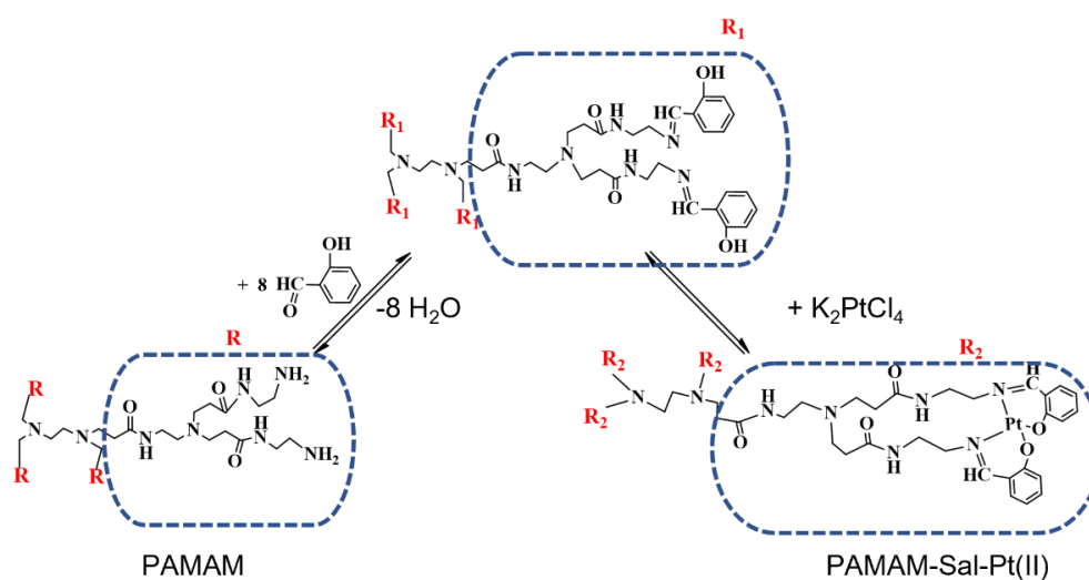
Fig. 1. Synthesis schematic of PAMAM-Sal-Pt(II)
