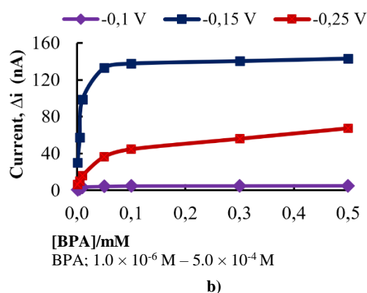
Fig. 6. (a) Amperometric response of CPE and MCPE to BPA. (b) Effect of working potential on the BPA sensitivity of MCPE (0.1 M, pH 7.0 phosphate buffer, 25 °C)
