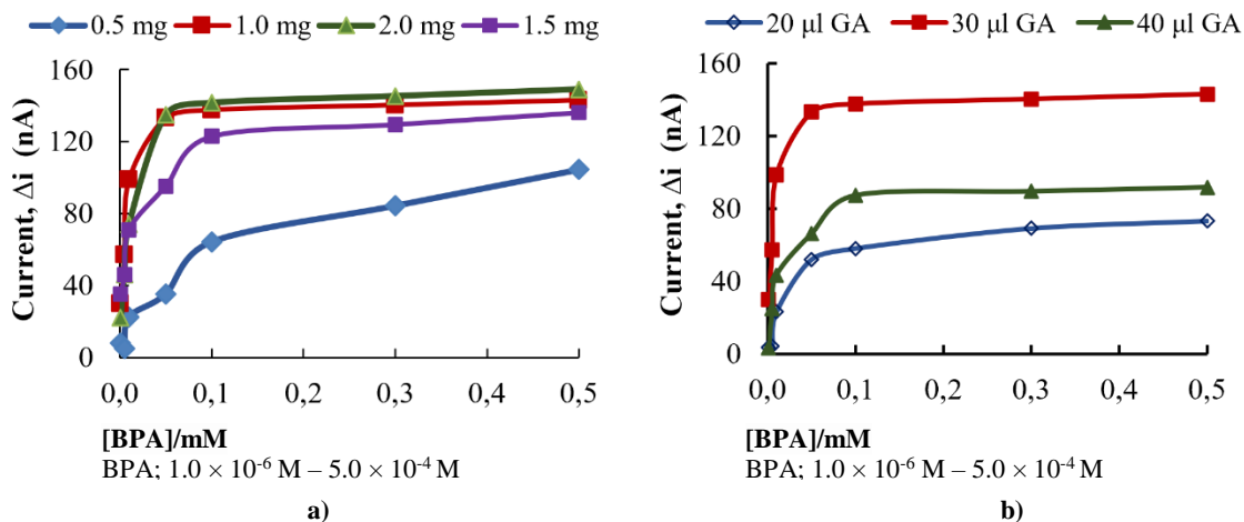
Fig. 7. (a) Effect of the amount of PAMAM-Sal-Pt(II) on the BPA sensitivity of MCPE (b) Effect of the amount of glutaraldehyde (2.5% glutaraldehyde solution was used)
