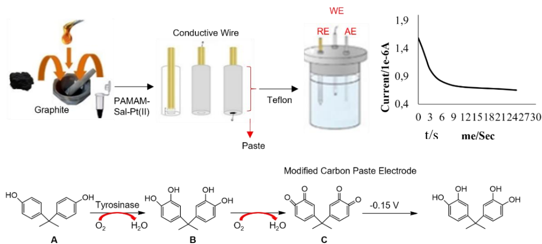
Fig. 2. Preparation of the MCPE and working cell scheme (A: 4,4'-(propane-2,2diyl)diphenol; BPA, B: 4,4'-(propane-2,2diyl)bisbenzo-1,2-diol, C: 4,4'-(propane-2,2diyl)biscyclohexane-3,5-diene-1,2-dione)
