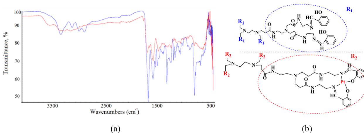
Fig. 4. (a) FT-IR spectra and (b) proposed of structures [PAMAM-Sal] and [PAMAM-Sal-Pt(II)]
