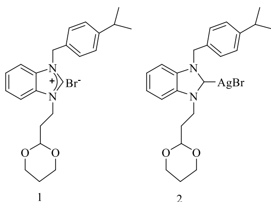
Fig. 1. Chemical structure of the synthesized compounds 1 and 2
