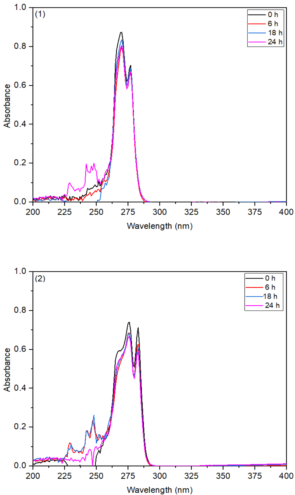
Fig. 7. UV spectra of compounds 1 and 2 in DMF at different time intervals
