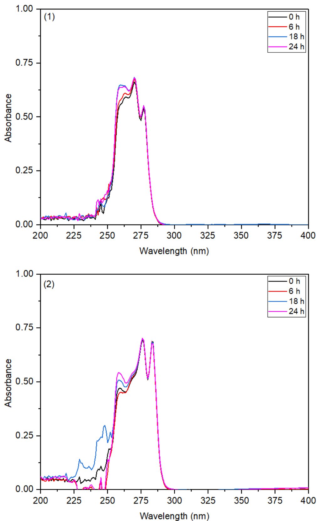
Fig. 6. UV spectra of compounds 1 and 2 in DMSO at different time intervals
