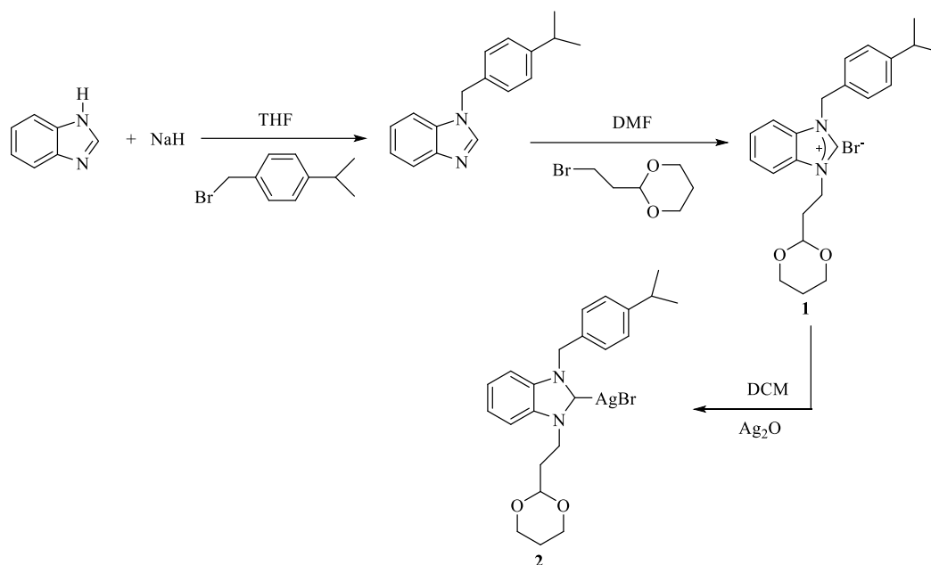
Fig. 2. General synthesis of compounds 1 and 2
