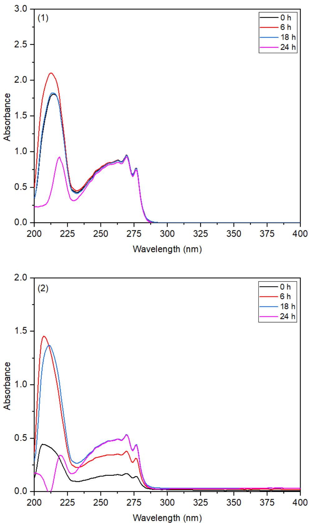
Fig. 5. UV spectra of compounds 1 and 2 in PBS at different time intervals
