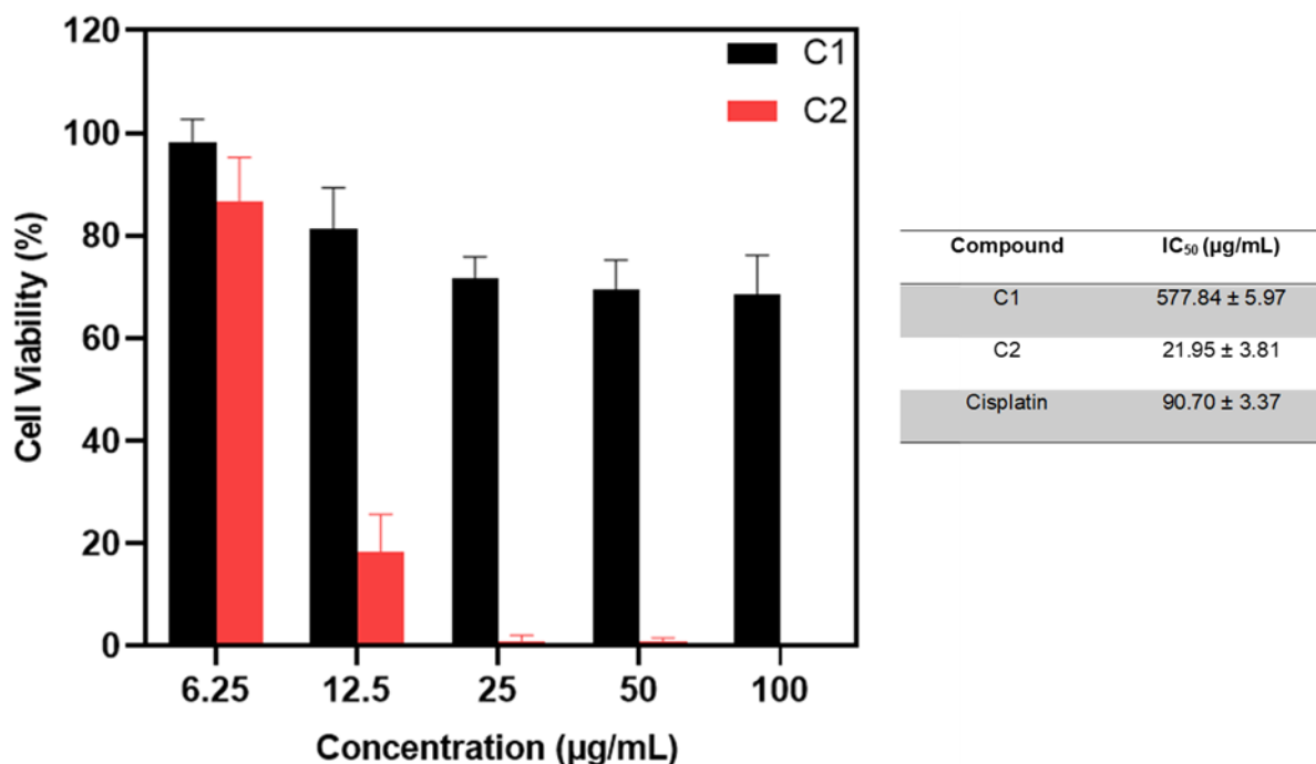
Fig. 3. The percentage cell viability of investigated compounds towards human colon cancer (HCT-116) and their \text{IC}_{50} values in \mu\text{g/ml} (inset)
