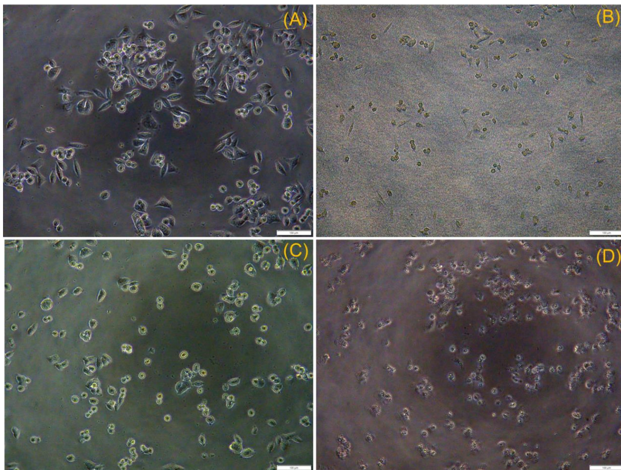
Fig. 4. Optical microscopy images of HCT-116 cell morphology (A) control, (B) DMSO, (C) compound 1 , and (D) compound 2 after 24 h of incubation
