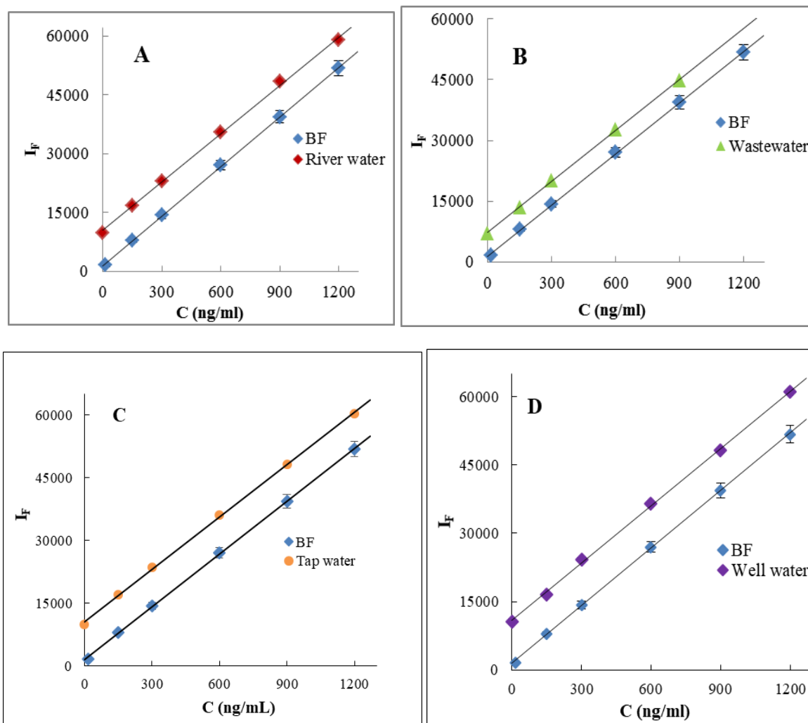
Fig 7b. Standard addition curves of BF pure samples in river water (A), in waste water (B) in tap water (C) and in well water (D)
