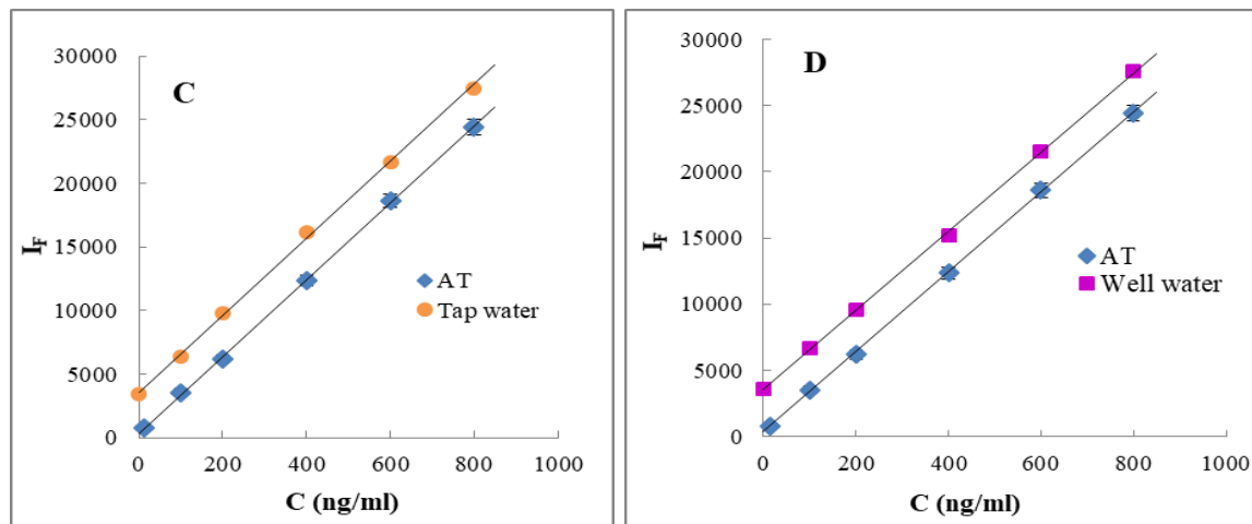
Fig 7b. Standard addition curves of BF pure samples in river water (A), in waste water (B) in tap water (C) and in well water (D)
