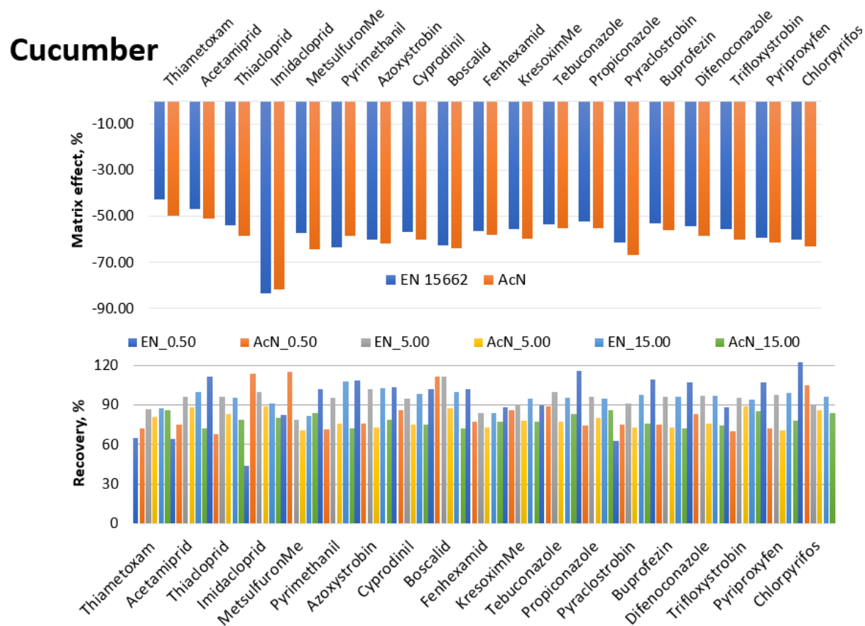
Figure S3. Matrix effects and recoveries at three spike levels (0.50, 5.00 and 15.00 mgkg -1 ) in cucumber treated with EN 15662 and AcN method
