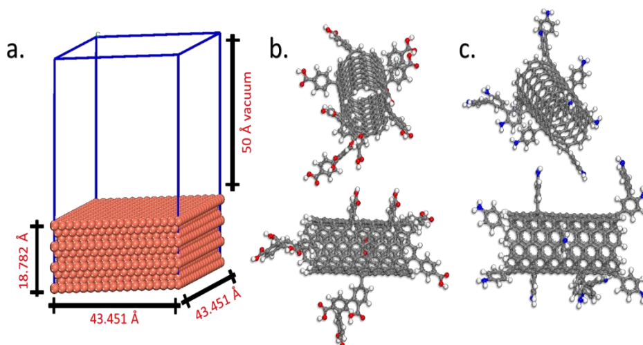
Fig. 1. Molecular models used in the theoretical calculations: a) Cu(111) facet, b) SWCNT-PhCOOH, and c) SWCNT-PhNH 2
