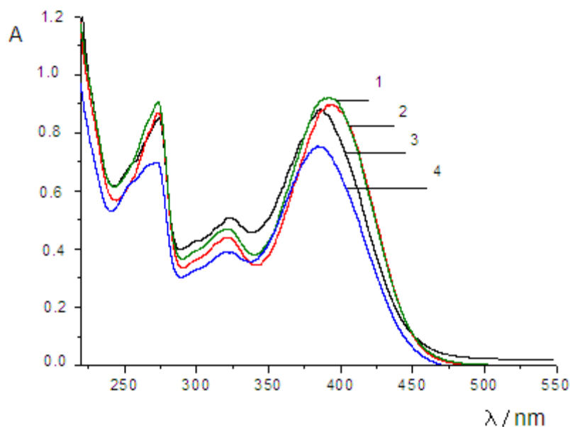
Fig. 3. UV-Vis absorption spectra of QR ( c_{\text{QR}} = 5 \cdot 10^{-5} \text{ mol l}^{-1} ) in the presence of CTAB in different methanol-water mixtures (v/v): 5 % (1), 10 % (2), 15 % (3), and 20 % (4); pH = 6.0; c_{\text{CTAB}} = 2 \cdot 10^{-3} \text{ mol l}^{-1}
