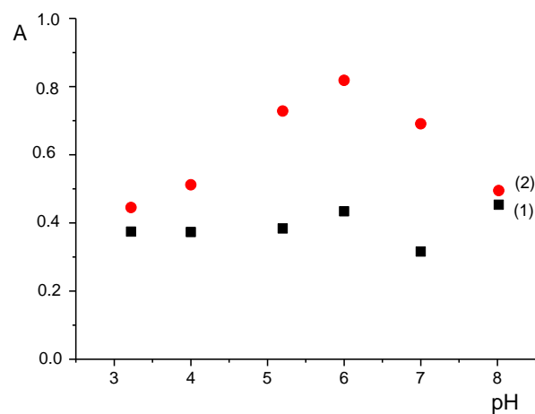
Fig. 4. The absorbance of 5 % methanolic solutions of QR ( c_{\text{QR}} = 4 \cdot 10^{-5} \text{ mol l}^{-1} ) in the absence (1) and the presence (2) of CTAB micelles at various pH values; \lambda = 397 \text{ nm} and c_{\text{CTAB}} = 2 \cdot 10^{-3} \text{ mol l}^{-1}
