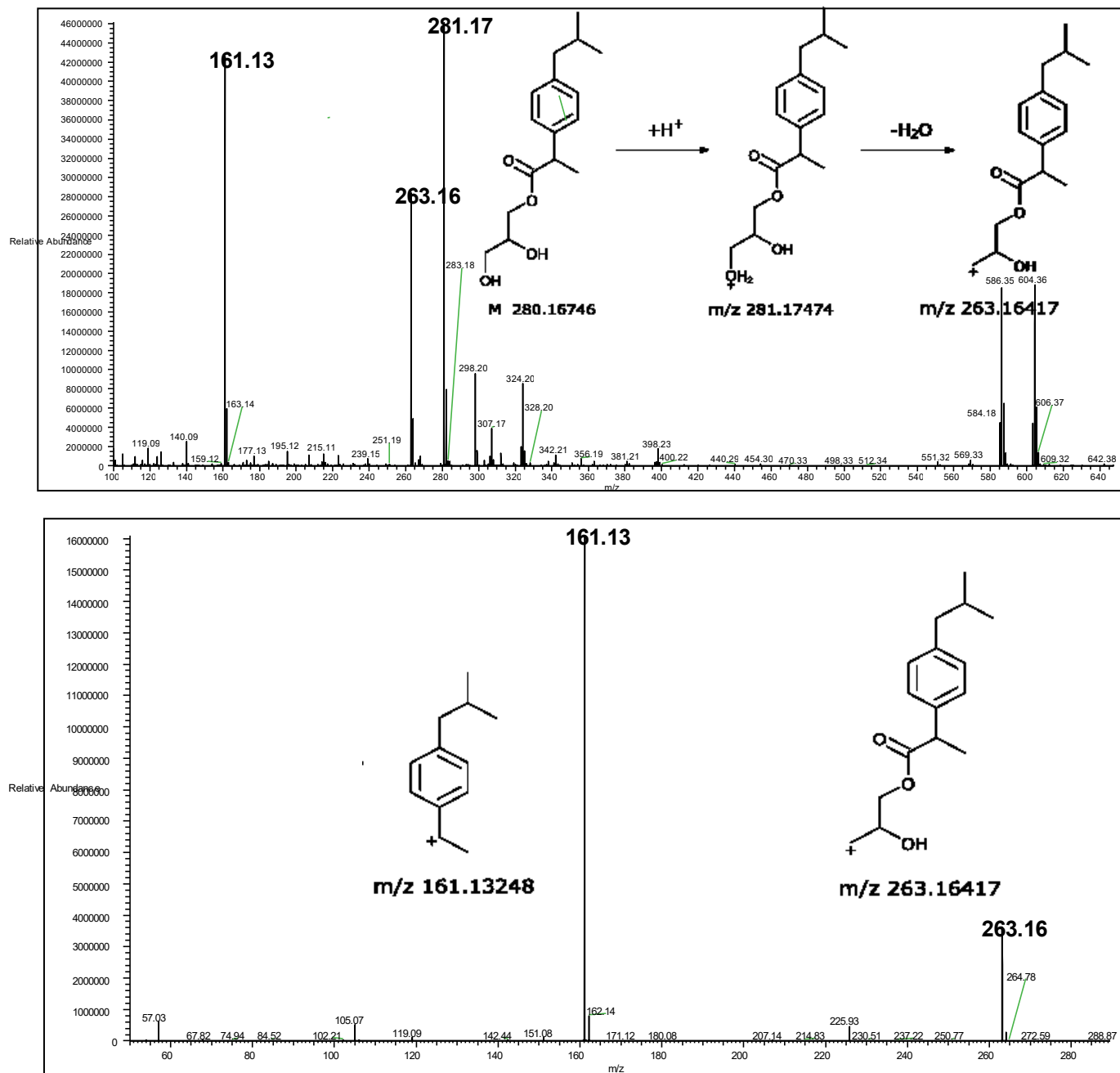
Fig. 4. Mass spectra collected for the peak of the major product P1. Top: full MS spectrum; Bottom: MS 2 spectrum from the peak at m/z 263
