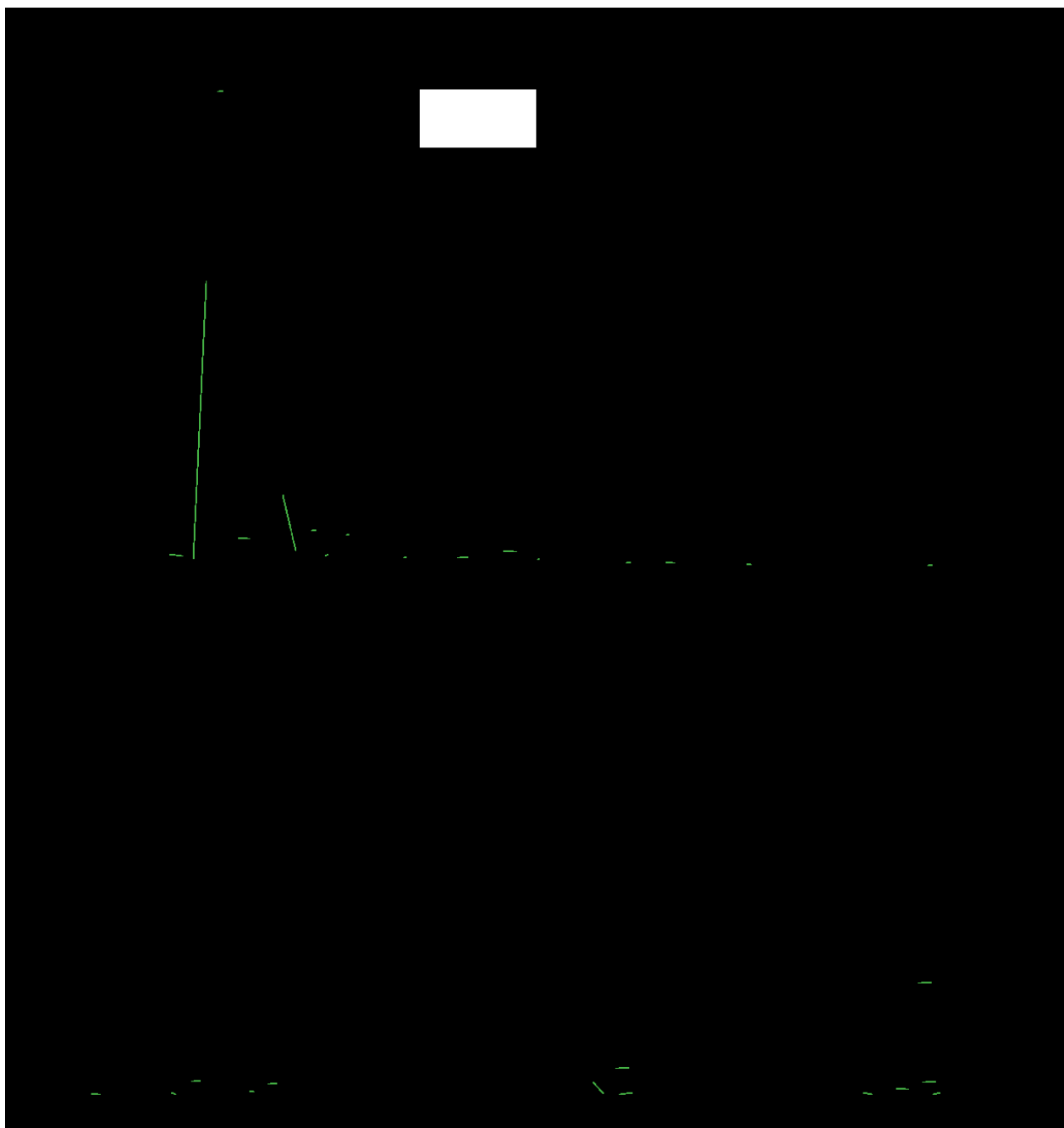
Fig. 3. Mass spectra collected from the peak of ibuprofen. Top: full MS spectrum; Bottom: MS 2 spectrum from the molecular ion [M+18 amu adduct]
