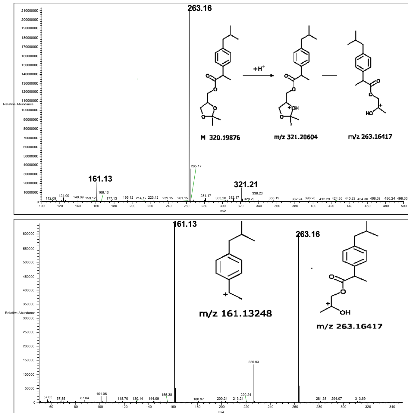
Fig. 6. Mass spectra collected from the peak P2. Top: full MS spectrum; Bottom: MS 2 spectrum from the peak at m/z 321
