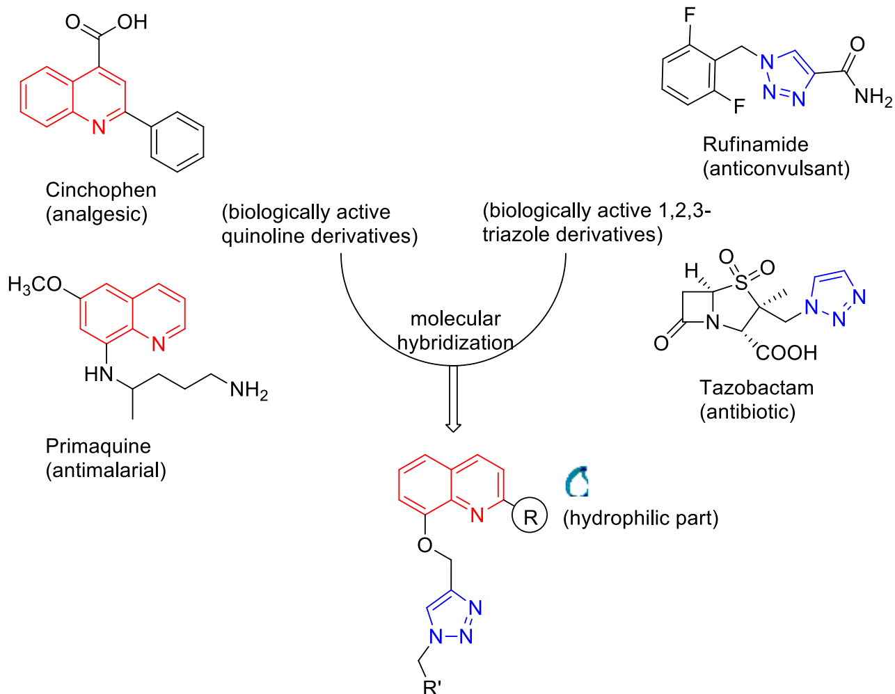
Fig. 1. Design of novel water-soluble quinoline-triazole hybrids
