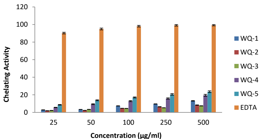
Fig. 3. Metal chelating activity of the synthesized compounds
