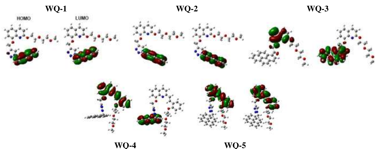
Fig. 8. HOMO and LUMO orbitals of WQ-1 , WQ-2 , WQ-3 , WQ-4 , and WQ-5
