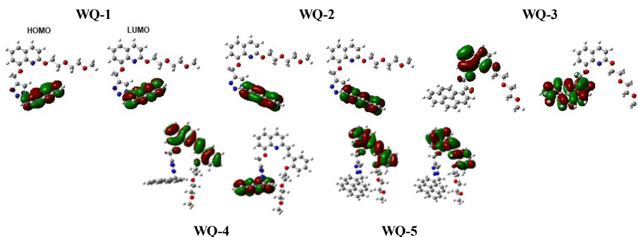
Fig. 8. HOMO and LUMO orbitals of WQ-1 , WQ-2 , WQ-3 , WQ-4 , and WQ-5
