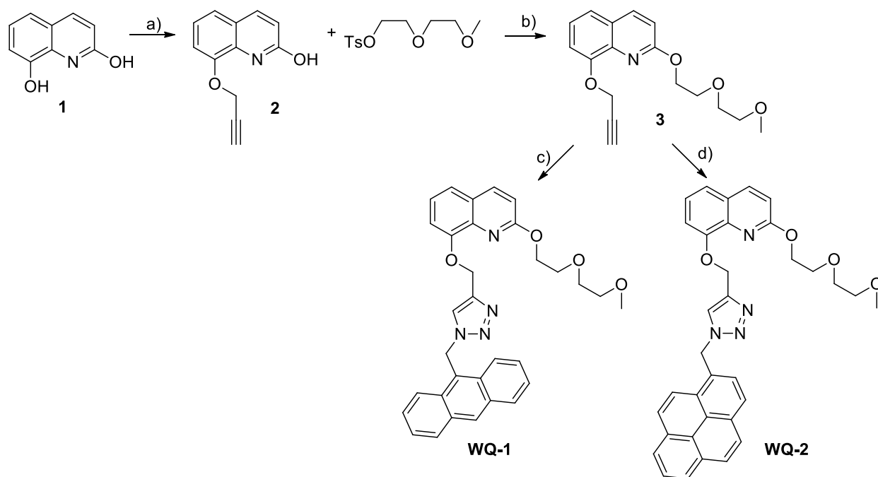
Scheme 1. a) Propargyl bromide, K 2 CO 3 , acetone; b) K 2 CO 3 , CH 3 CN; c) 9-(azidomethyl)anthracene, CuSO 4 , sodium ascorbate, THF:H 2 O; d) 1-(azidomethyl)pyrene, CuSO 4 , sodium ascorbate, THF:H 2 O
